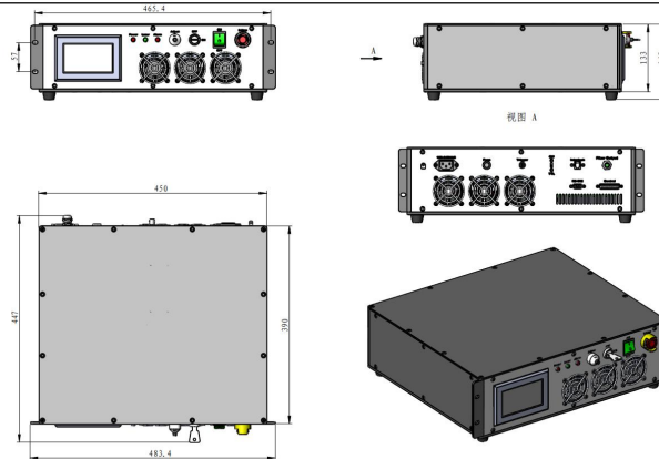
FC-W-445C (Air Cooled)
