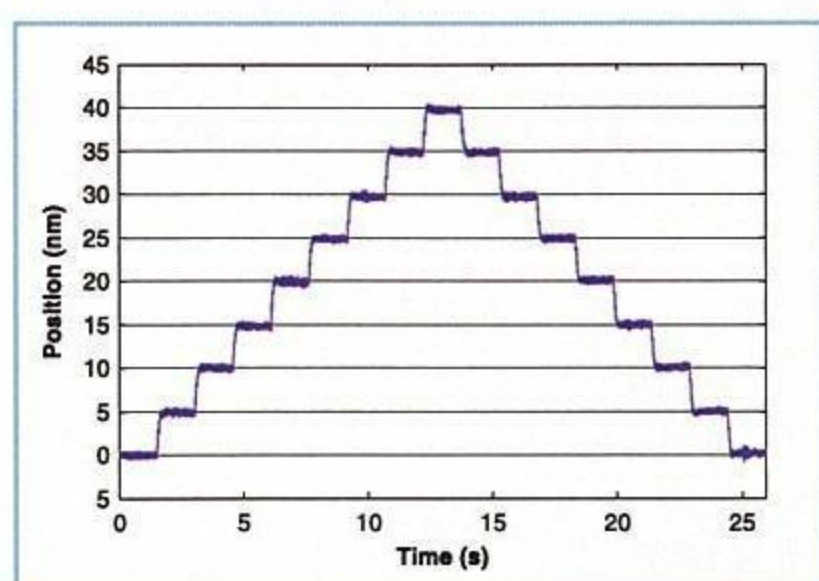
ANT95-50-L-PLUS 5 nm step plot
