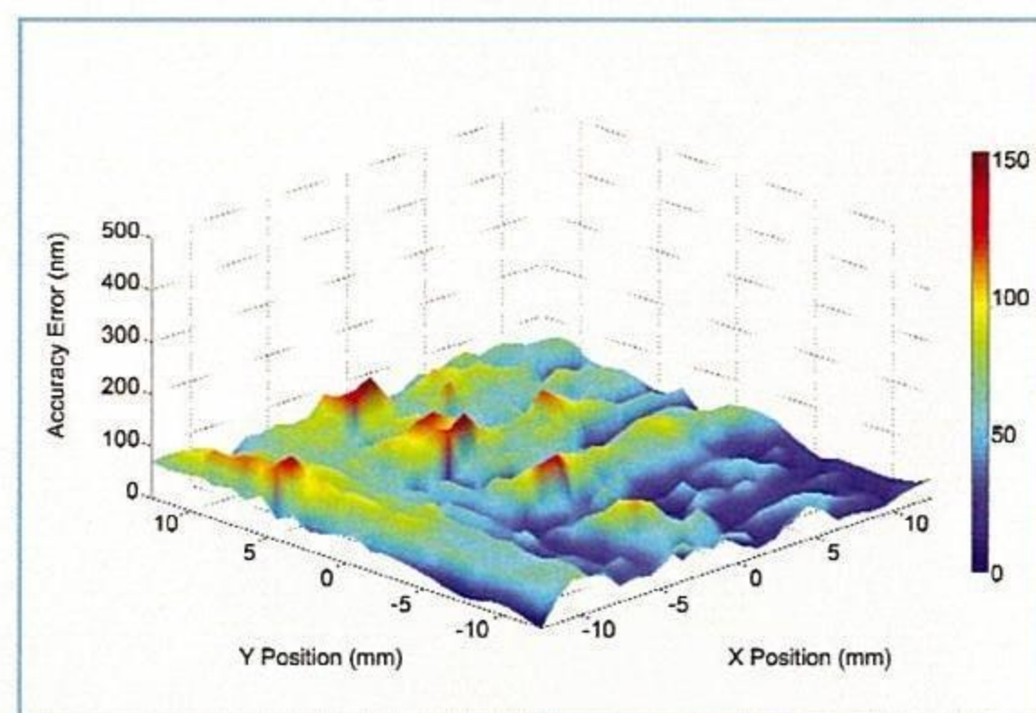
ANT95-XY ULTRA 2D accuracy
