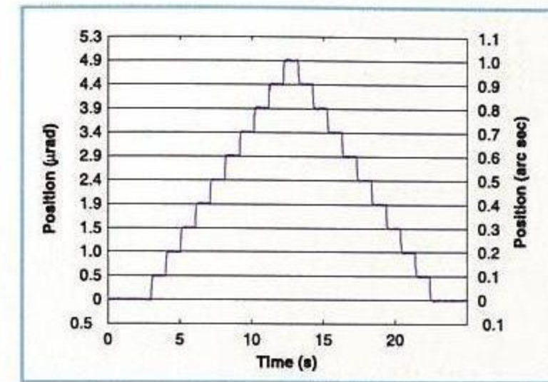
ANT95-R 0.10 arc-sec step plot
