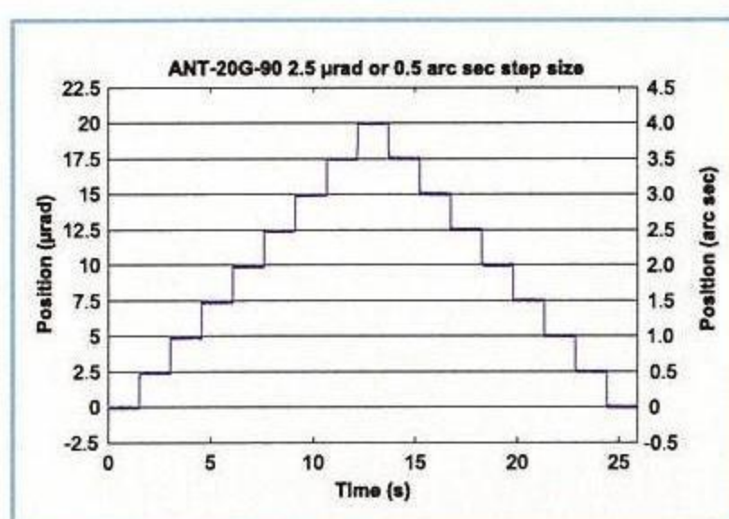
ANT-20G-90 0.5 arc-sec step plot
