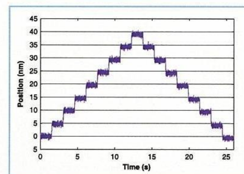
ANT130-60-L-PLUS 5 nm step plot
