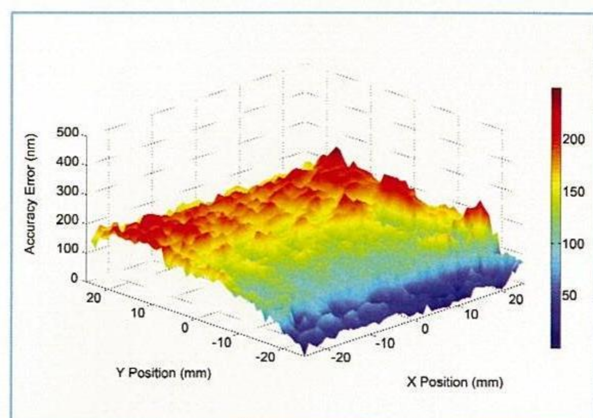
ANT130-XY ULTRA 2D accuracy
